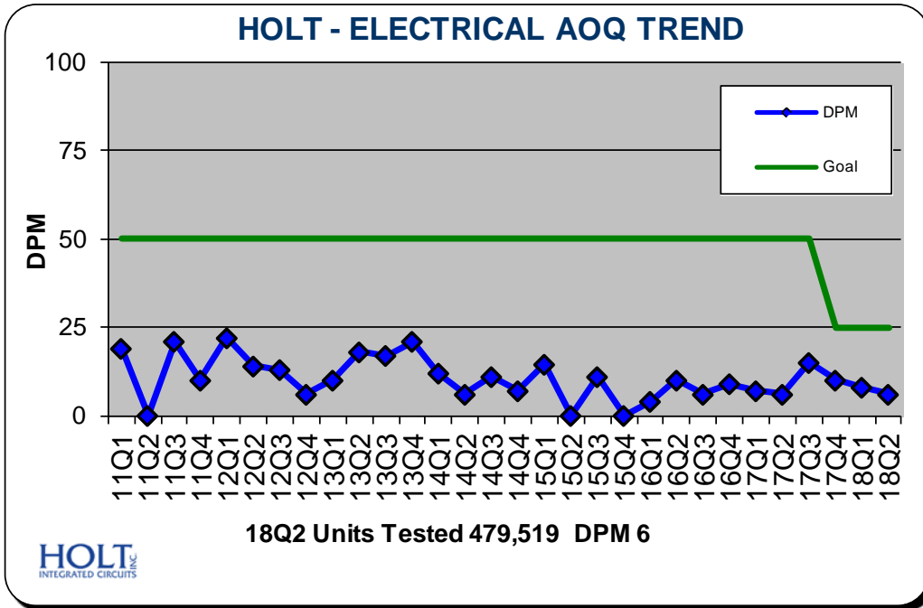
Figure 2 –Electrical AOQ
