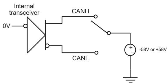
Figure 16. CAN Bus Driver Short-Circuit Test
