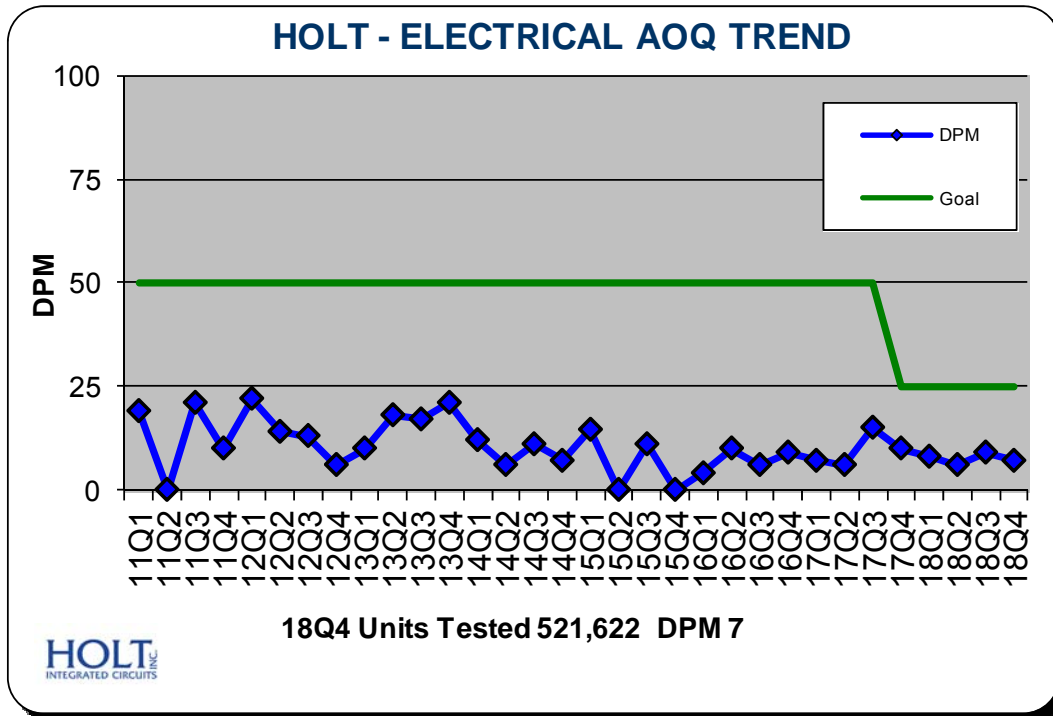
Figure 2 –Electrical AOQ
